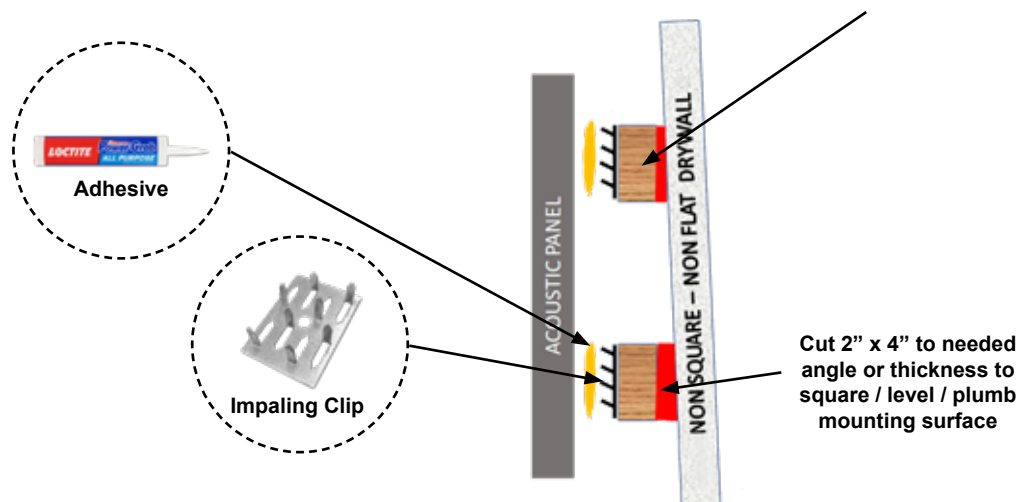
2" x 4" Nominal Furring Strip
